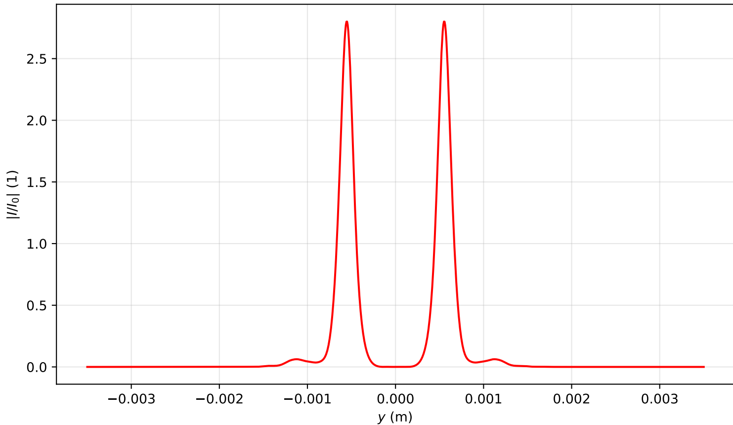
Intensity profile I(x=0, y, z=0.716)/I_0 , P_{in}=9.0P_{cr} , artificial time
